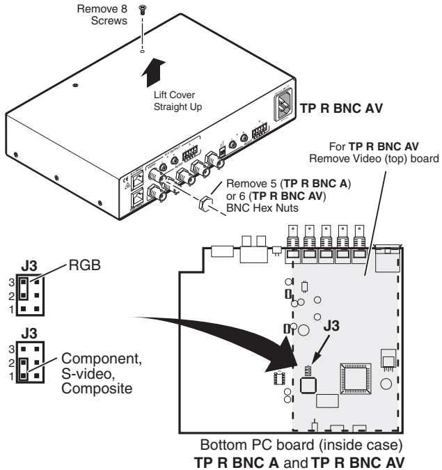
Figure 2-1 — Video jumper configuration
