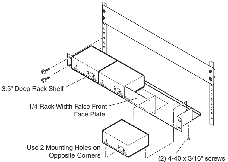
Figure 2-4 — Rack mounting the TP R 15HD A
