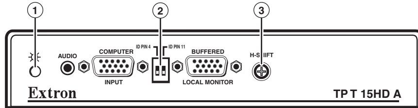
TP T 15HD A front panel
