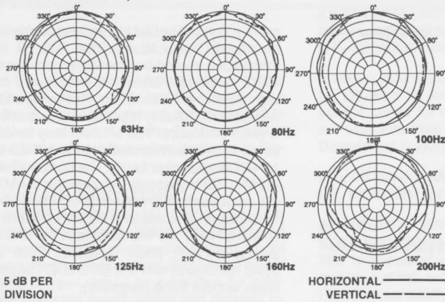
FIGURE 3 — Polar Response
