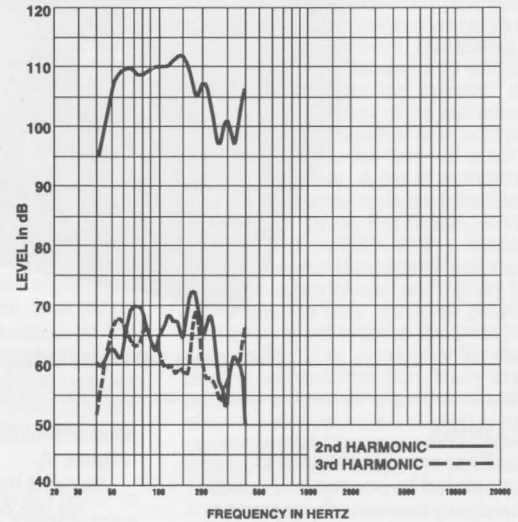
FIGURE 6 — Harmonic Distortion
