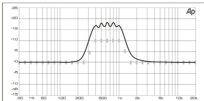
Graphic EQ without frequency response correction.
