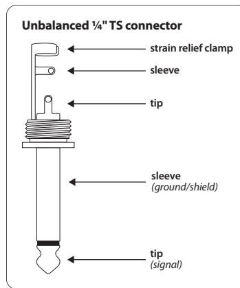
Fig. 3.3: 1/4" TS connector
