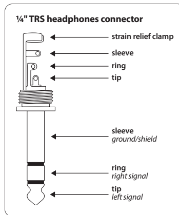
Fig. 3.5: 1/4" headphones connector
