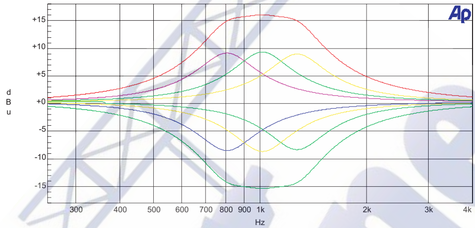
Figure 3 Symmetrical-Q equaliser "wide" mode full boost and cut
