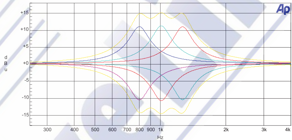
Figure 4 Symmetrical-Q equaliser "narrow" mode full boost and cut
