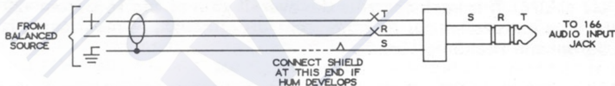
Figure 1: Balanced sources
